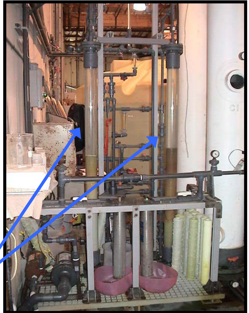
Chromium Specific Ion Exchange Columns
